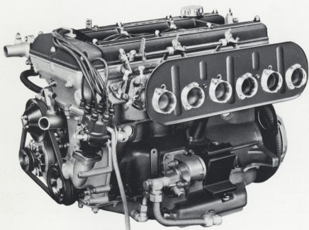
FIG.-6 ENGINE ASSEMBLY (MF10)
