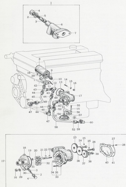
FIG.-16 OIL PUMP &amp; OIL REGULATOR
