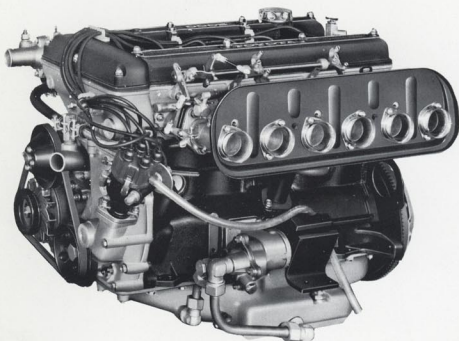
FIG.-7 ENGINE ASSEMBLY (MF10L)
