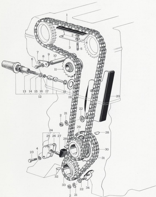
FIG.-15 TIMING CHIN &amp; DAMPER
