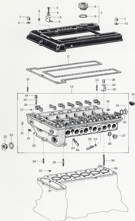
FIG.-9 CYLINDER HEAD &amp; HEAD COVER
