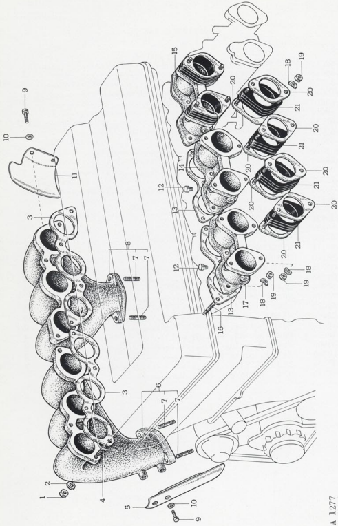
FIG. -21 MANIFOLD
