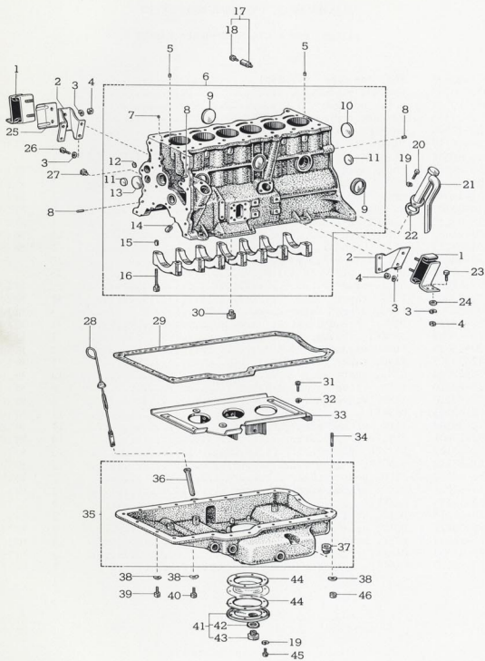
FIG.-10 CYLINDER BLOCK &amp; ENGINE MOUNTING
