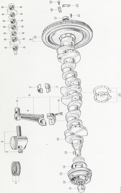
FIG.-12 CRANKSHAFT & CONNECTING ROD
