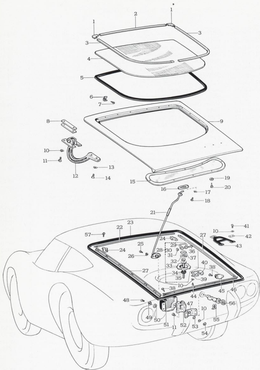
FIG.-112 BACK DOOR PANEL &amp; DOOR LOCK
