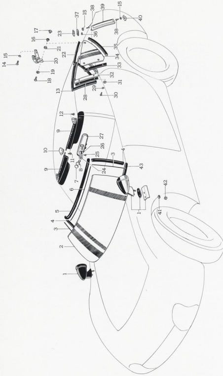
FIG.-114 FRONT WINDOW GLASS & QUARTER WINDOW
