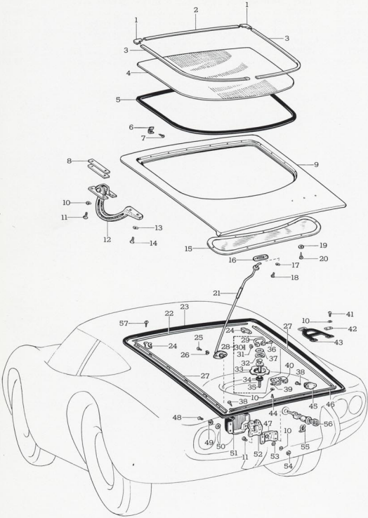
FIG.-112 BACK DOOR PANEL & DOOR LOCK
