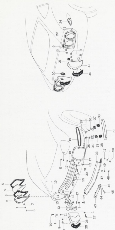
FIG.-104 BUMPER &amp; RADIATOR GRILLE
