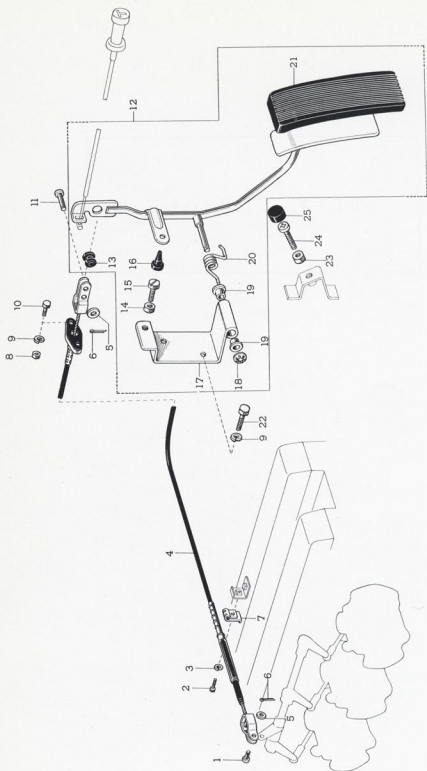
FIG.-101 ACCELERATOR LINK (MF10)
